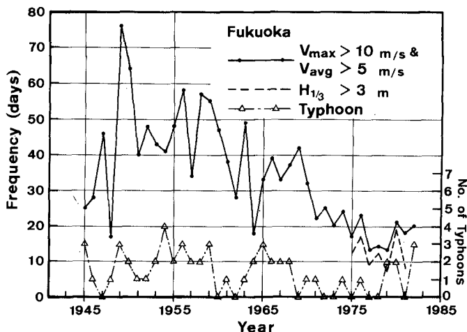
Figure 8 Frequencies of Storm winds, Waves and Typhoons
