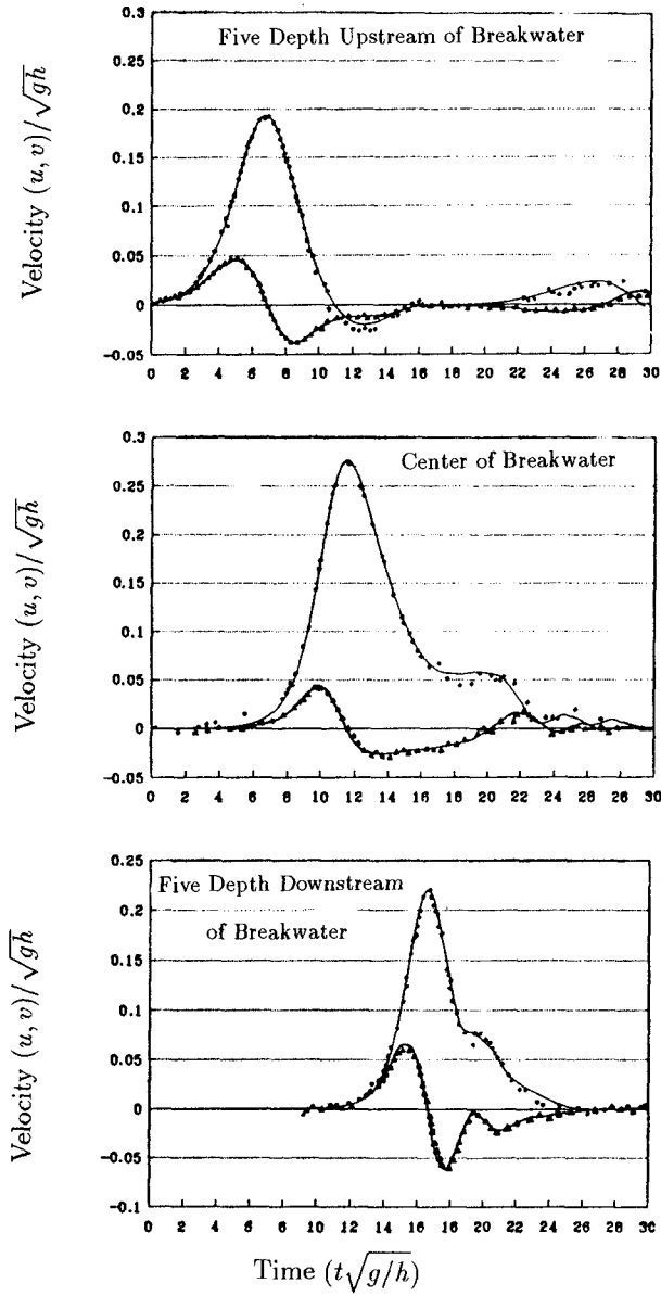
Figure 4: Comparison of water particle velocities at three different locations (— present theory; \cdots experiment, u component; \triangle\triangle\triangle experiment, v component)
