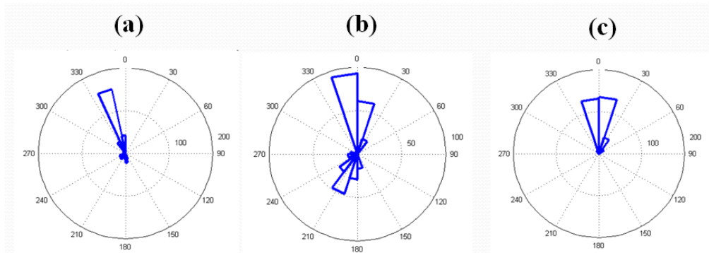
Figure 10 . The wind rose at 200 meters of three typhoon events (a) Typhoon Soulik from July 11 to July 13,2013 (b) Typhoon Trami from August 20 to August 22,2013 (c) Typhoon Fitow from October 4 to October 7, 2013.
