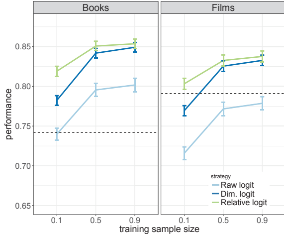
Figure 3: Average performance of the various logit strategies at the individual level when the models were trained with 10%, 50%, and 90% percent of the data (20, 100, and 180 choices, respectively). The dashed horizontal lines show the performance of the neural network trained on the aggregate data. With individual-level data, the models outperformed their aggregate-level counterparts by more than 10% in the case of books and 5% in the case of films.
