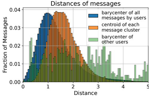
Figure 3: Distributions of Euclidean distances in the curiosity stimulus space between the messages sent by a user and (i) the barycenter of all messages by the same user (blue), (ii) the centroid of each message’s profile (orange) and (iii) the barycenter of messages sent by other users in the last 15 minutes (green).
