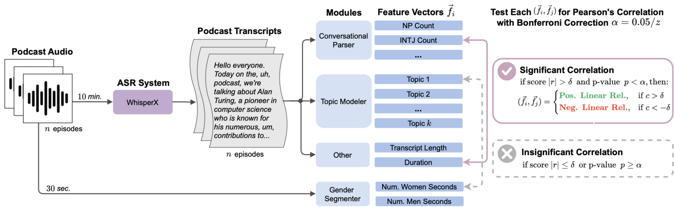
Figure 2: GDCF (Gendered Discourse Correlation Framework) Diagram: Testing for correlations with an example of a significant correlation and an insignificant correlation – all (\vec{f}_i, \vec{f}_j) pairs are labeled significant or insignificant . |\vec{f}_i| = 15,117 podcast episodes. z = \binom{124}{2} = 7,626 correlation tests for the 124 total feature vectors.
