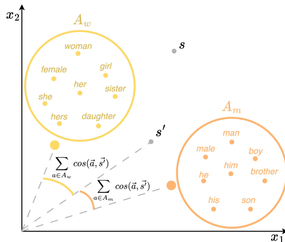
Figure 1: An overview of our two-part framework: (i) Using our Gendered Discourse Correlation Framework (GDCF, as shown in Figure 2), we obtain gendered discourse word lists . (ii) We then perform our Discourse Word-Embedding Association Test (D-WEAT, as shown here in Figure 1). We form parallel sentences, s and s' , by swapping masculine discourse words (e.g. “going”) for feminine discourse words (e.g. “like”): s = \text{And I was } \mathbf{going}, \text{ hey, it's cold outside...} , and s' = \text{And I was } \mathbf{like}, \text{ hey, it's cold outside...} . We find that the masculine discourse words have a more stable embedding representation – this is a representational harm and a masculine default.
