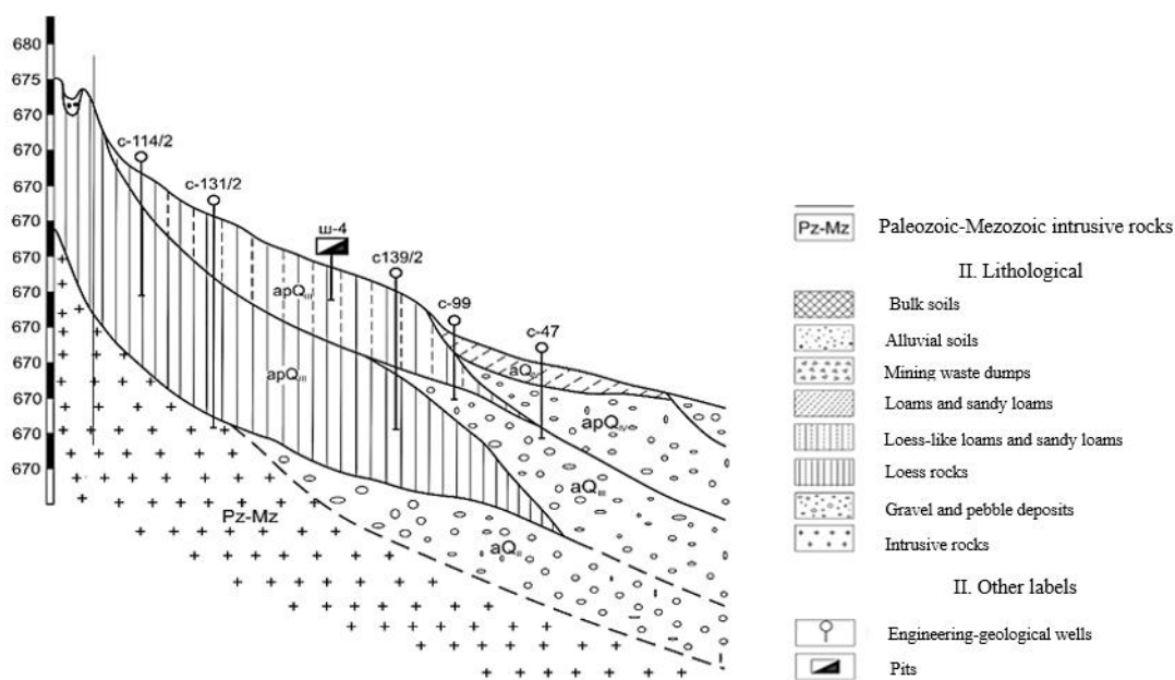
Fig.2 Engineering-geological section of the city of Olmaliq
