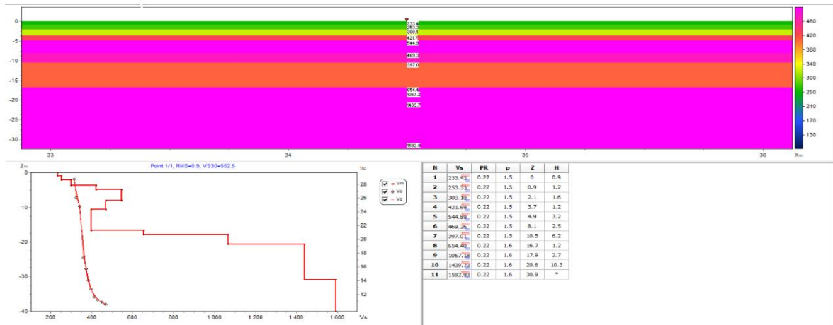
Fig. 3. Depth-velocity model of transverse waves according to MASW. Profile 1 shear wave velocity model ии MASW. Profile 1. ( tab. 1 )
