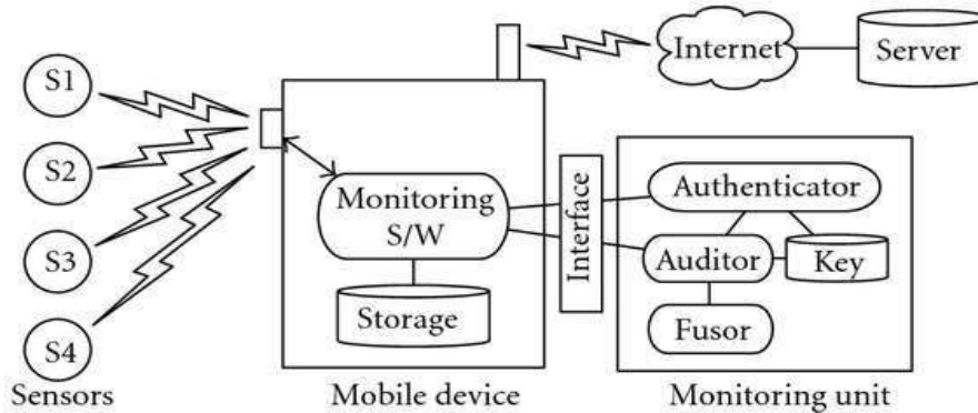
Figure 1: Health monitoring architecture.
