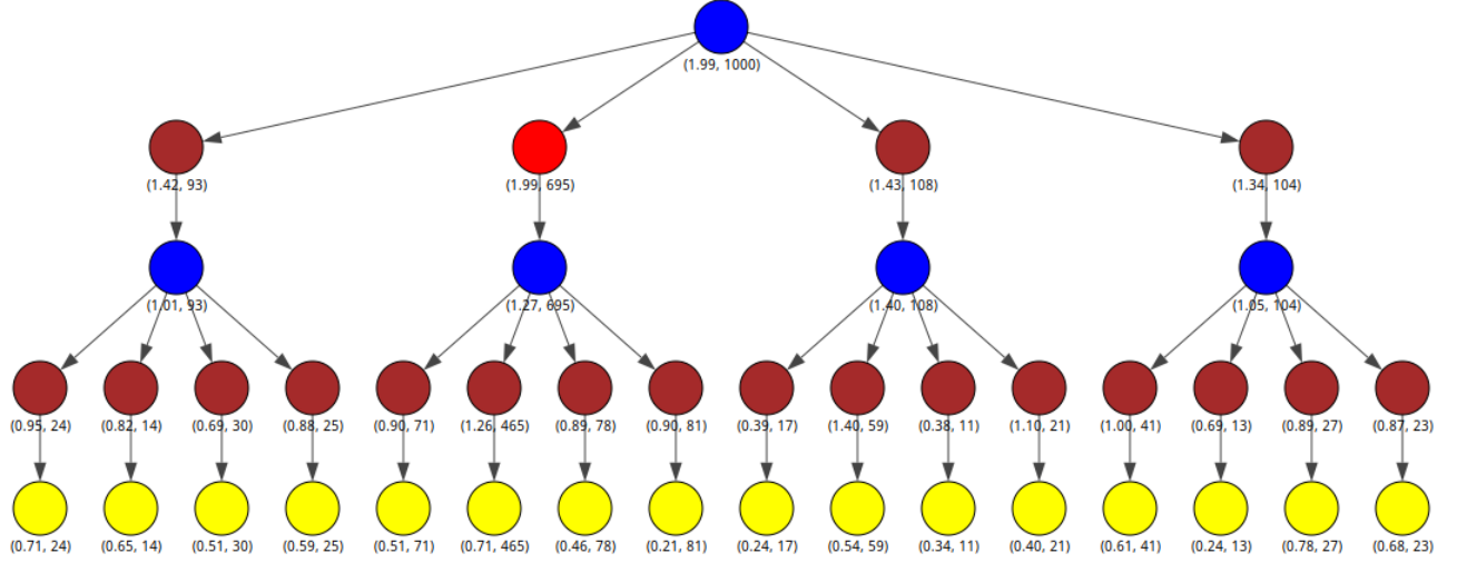
(a) MENTS.
