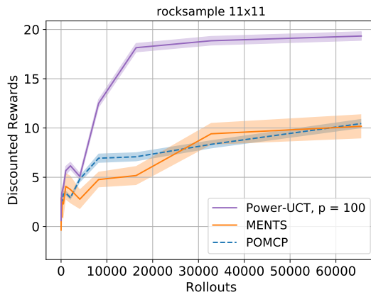
Figure 6: Performance of Power-UCT compared to UCT and MENTS in rocksample 11x11. The mean of discounted total reward over 1000 evaluation runs is shown by thick lines while the shaded area shows standard error.
