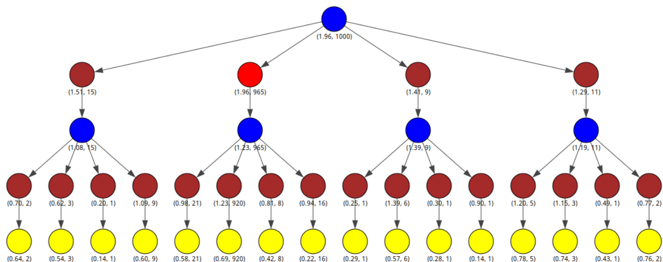
(b) Power-UCT.
