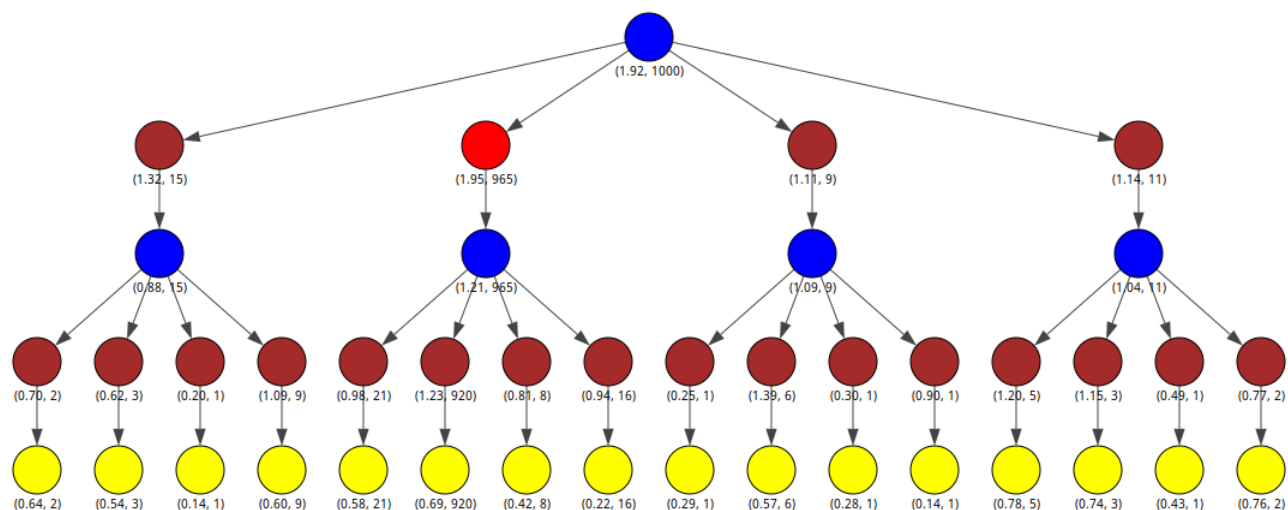
(a) UCT.
