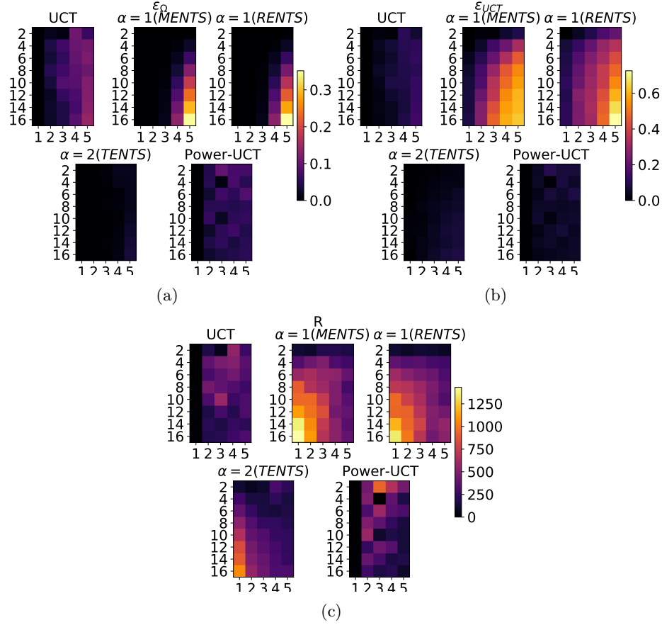
Figure 7: For different branching factor k (rows) and depth d (columns), the heatmaps show: the absolute error of the value estimate at the root node after the last simulation of each algorithm w.r.t. the respective optimal value (a), and w.r.t. the optimal value of UCT (b); regret at the root node (c).
