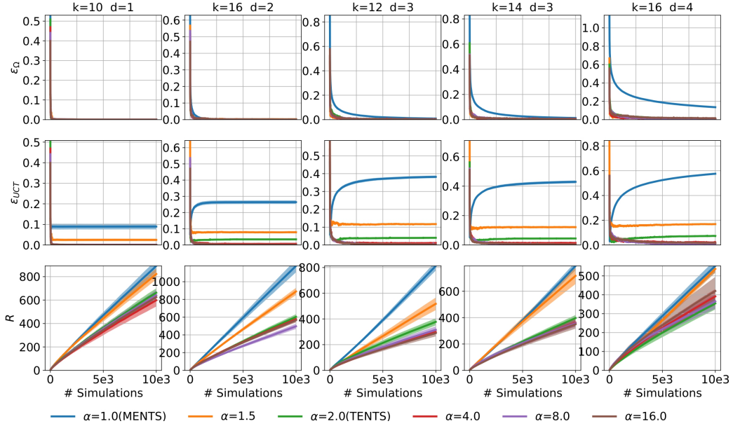
Figure 12: We show the convergence of the value estimate at the root node to the respective optimal value (top), to the UCT optimal value (middle), and the regret (bottom) with different \alpha parameter of \alpha -divergence in Synthetic tree environment with \alpha = 1.0 (MENTS), 1.5, 2.0 (TENTS), 4.0, 8.0, 16.0.
