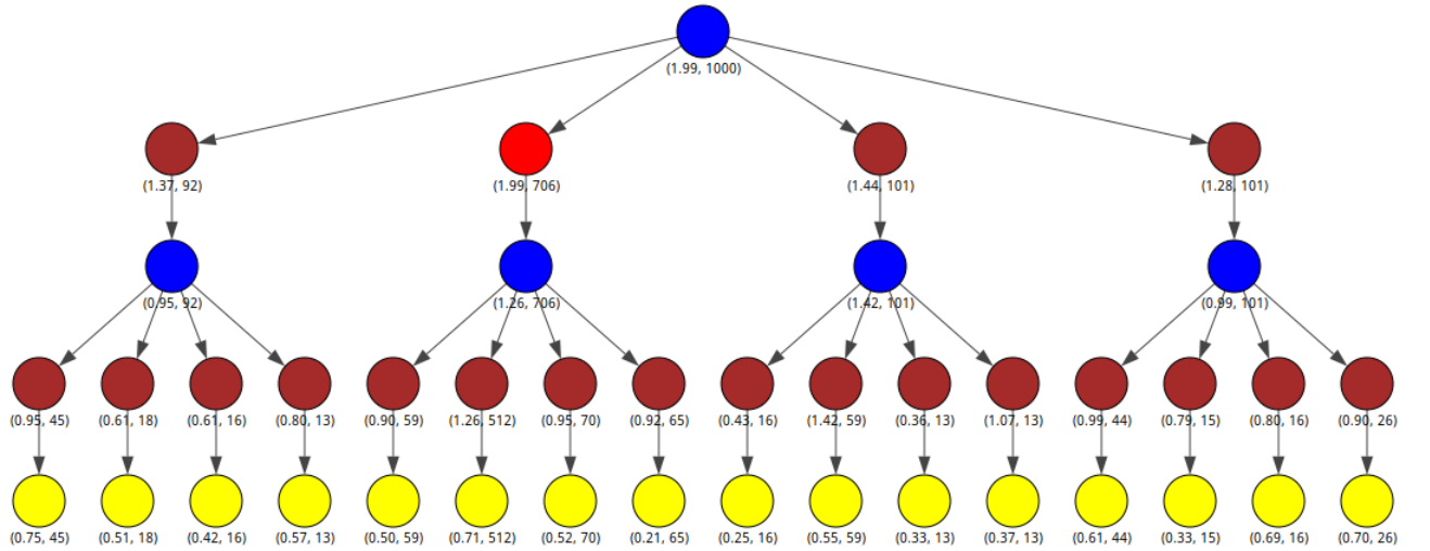
(b) TENTS.
