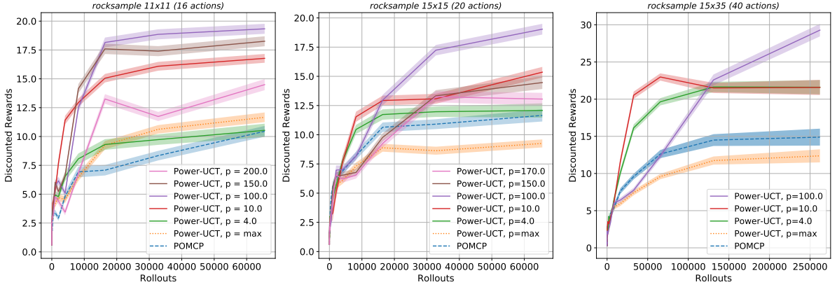
Figure 5: Performance of Power-UCT compared to POMCP in rocksample . The mean of total discounted reward over 1000 evaluation runs is shown by thick lines while the shaded area shows standard error.
