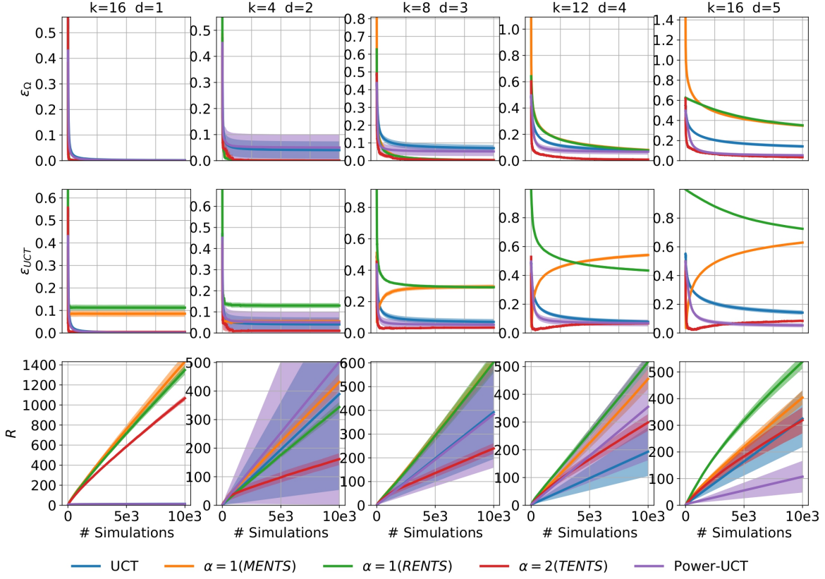
Figure 9: For each algorithm, we show the convergence of the value estimate at the root node to the respective optimal value (top), to the UCT optimal value (middle), and the regret (bottom).
