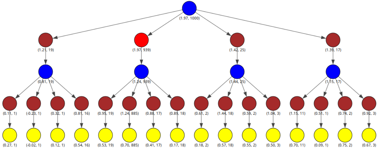
Figure 16: Monte-Carlo Tree Search of \alpha -divergence( \alpha = 4.0 ) and \alpha -divergence( \alpha = 8.0 ) after 1000 samples. Blue color circle is Vnode, Brown color circle is Qnode. Yellow color circle is the leaf node. Red color circle is the node with the optimal Qvalue function. Labels below the circles are (empirical mean value, visitation count). The optimal action selection in \alpha -divergence( \alpha = 8.0 ) converges faster than \alpha -divergence( \alpha = 4.0 ) as we can see at the optimal node in red color, the number of visitation in the tree of \alpha = 4.0 is 921 compared to 939 of \alpha = 8.0 .
