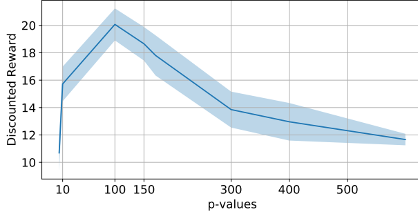
Figure 4: Evaluating Power-UCT w.r.t. different p -values: The mean discounted total reward at 65536 simulations (shaded area denotes standard error) over 100 evaluation runs.
