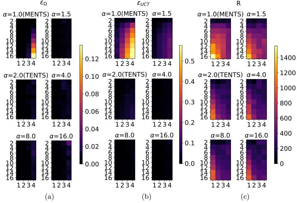
Figure 13: We show the effectiveness of \alpha -divergence in Synthetic Tree environment with different branching factor k (rows) and depth d (columns). The heatmaps show: the absolute error of the value estimate at the root node after the last simulation of each algorithm w.r.t. the respective optimal value (a), and w.r.t. the optimal value of UCT (b); regret at the root node (c).
