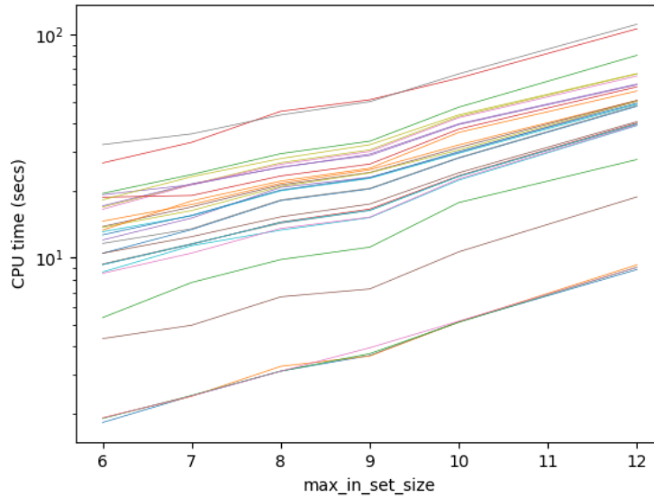
Fig. 19. CPU time dependence on maximum input set size for acceptability tuple discovery. Each line consists of a series of points each a single run of clingo using the default configuration, and applying acceptability tuple discovery on a single recipe. The x-position of each point shows the value of the max_input_set_size parameter for that run and the y-position is the CPU time for the execution. Y-axis is in log-scale to highlight the exponential relationship between independent and dependent variable.
