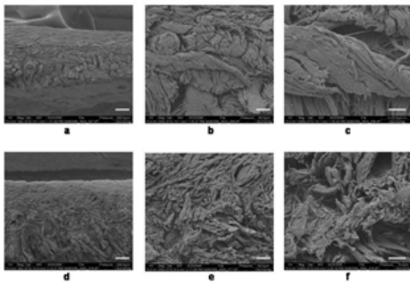
Figure 10: Scanning Electron Microscope images of blue stock from neck area: controls (treated with pH-adjusting agents alone) 100X ( \bar{=} 300 \mu\text{m} ) (a), 250X ( \bar{=} 50 \mu\text{m} ) (b), and 1000X ( \bar{=} 20 \mu\text{m} ) (c); filled blue stock, treated with gelatin/whye (2 units) 100X ( \bar{=} 300 \mu\text{m} ) (d), 250X ( \bar{=} 50 \mu\text{m} ) (e), and 1000X ( \bar{=} 20 \mu\text{m} ) (f).
