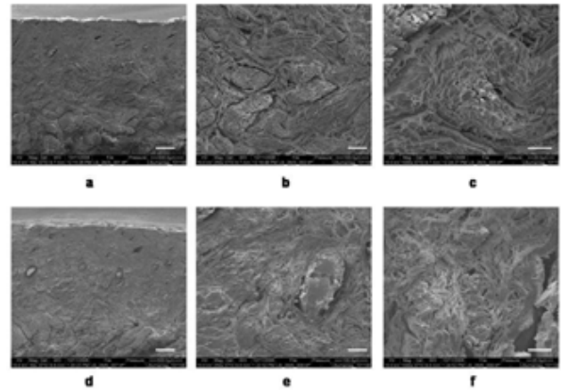
Figure 11: Scanning Electron Microscope images of retanned, colored, fatliquored blue stock from neck area: controls (treated with pH-adjusting agents alone) 100X ( \bar{=} 300 \mu\text{m} ) (a), 250X ( \bar{=} 50 \mu\text{m} ) (b), and 1000X ( \bar{=} 20 \mu\text{m} ) (c); filled blue stock, treated with gelatin/whye (2 units) 100X ( \bar{=} 300 \mu\text{m} ) (d), 250X ( \bar{=} 50 \mu\text{m} ) (e), and 1000X ( \bar{=} 20 \mu\text{m} ) (f).
