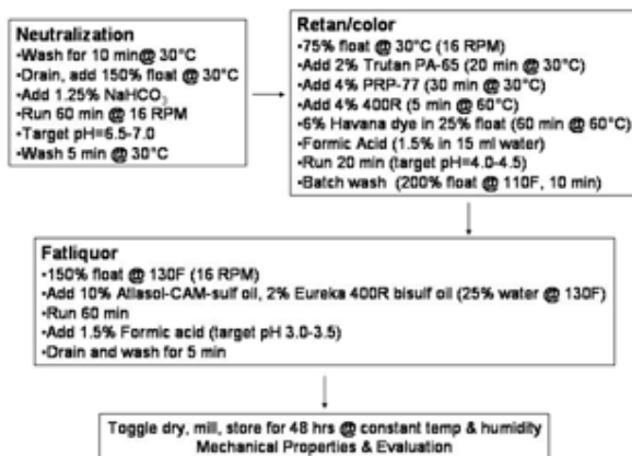
Figure 2: Flow diagram for retan, color and fatliquor of control and treated samples of blue stock.
