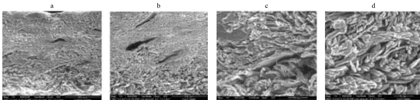
Figure 4: Scanning electron micrographs of finished leather samples showing the cross section at lower and higher magnifications a) control (x150) b) experimental (x150) c) control (x500) and d) experimental (x500)
