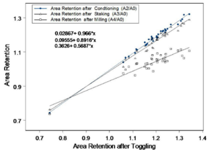
Figure 3. Area Retention after (a) conditioning, (b) staking and (c) drum milling
