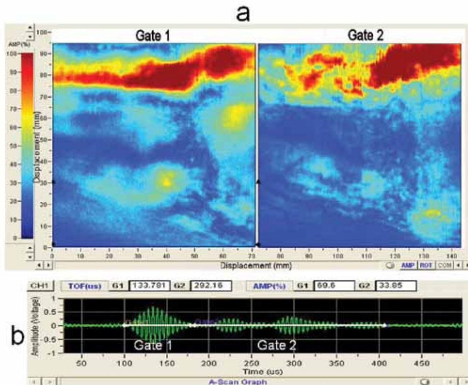
Figure 3. A typical (a) C-scan image and (b) A-scan graph in AU test.
