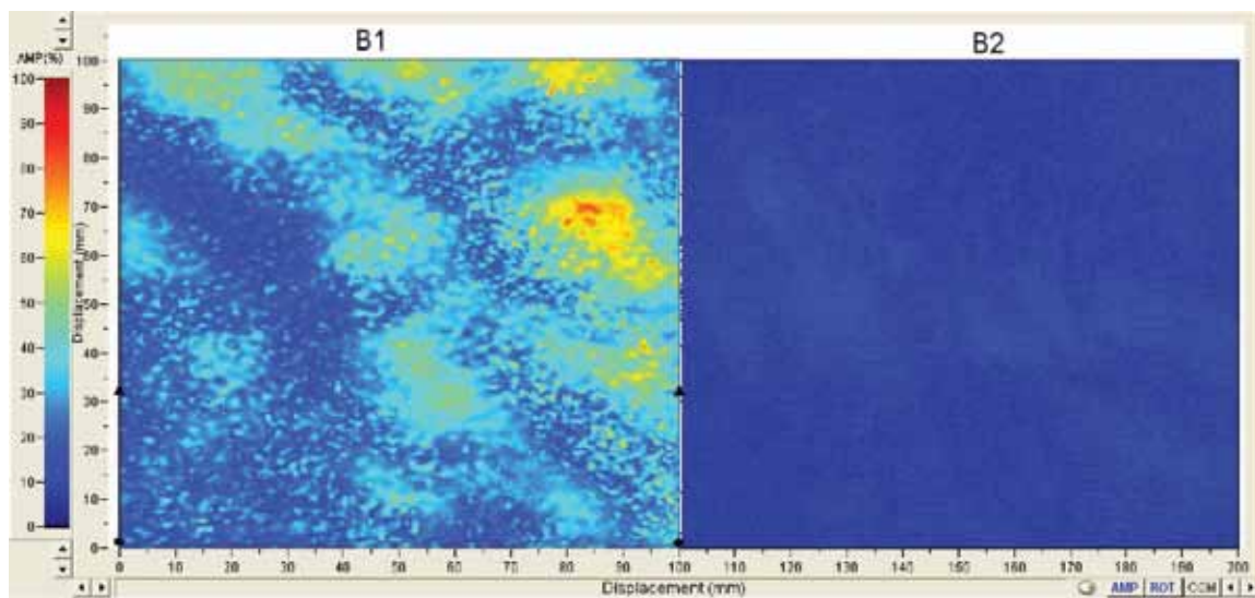
Figure 13. Amplitude C-scan images of different crust leather samples with vertical fiber defect.
