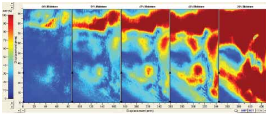
Figure 10. C-scan images of wet blue with brand at decreasing moisture levels: 61, 51, 47, 43, and 28%.
