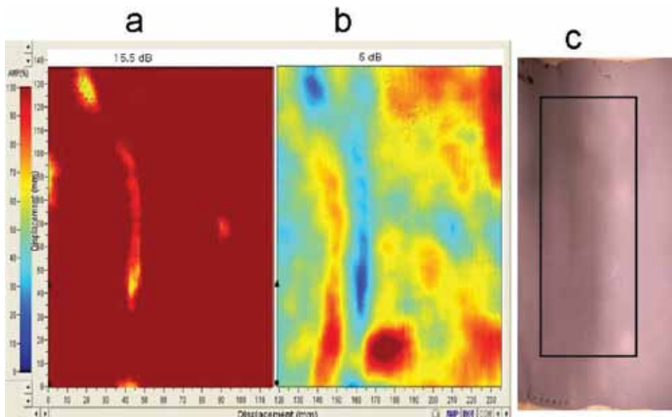
Figure 8. (a) C-scans from 15.5 dB gain, (b) 5dB gain, and (c) photo of wet blue.
