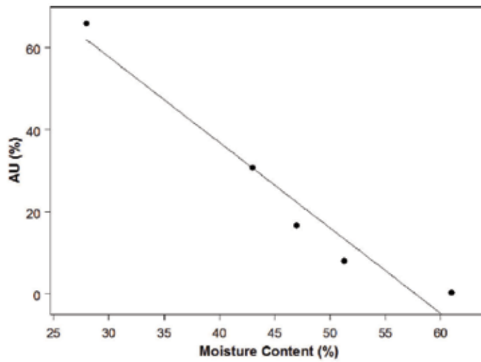
Figure 11. The relationship between percent area in 80-100% Amplitude range (AU%) and moisture content of wet blue.
