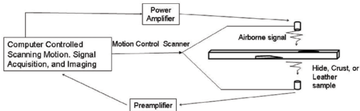
Figure 1. Schematic of airborne ultrasonic setup.
