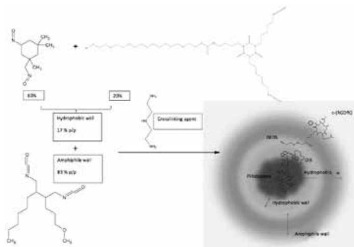
Figure 1. Amphiphile System for polymerization.
