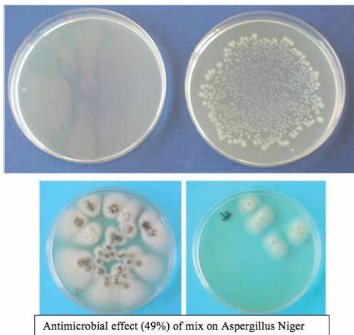
Figure 8. Blank sample showing growth and antimicrobial effect of mix.
