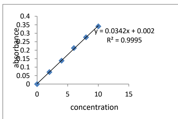
Fig.3: Standard curve of famotidine in 0.1 N HCl at 261 nm
