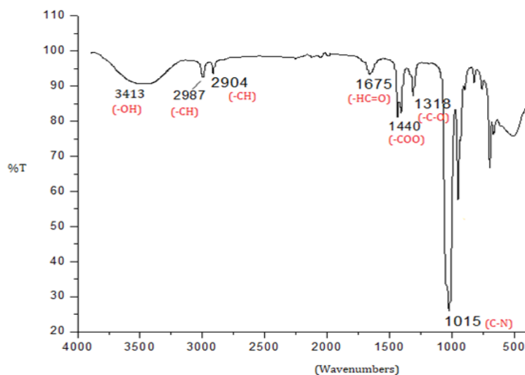
Fig 1 : FT-IR Spectra of CA 4 hydrogel
