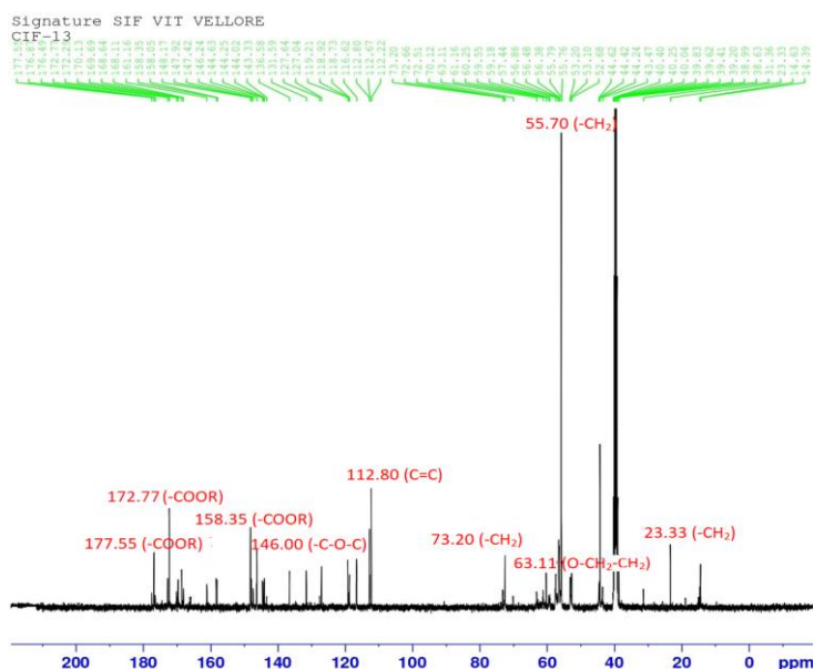
Fig 4 : ^{13}\text{C} NMR of CA 4 hydrogel
