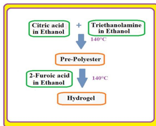
Scheme 1 : Synthesis of biopolymeric hydrogel
