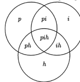
Fig. 1 Venn diagram of the interrelationship between influences in the Two-Facets design ( p \times i \times h )
