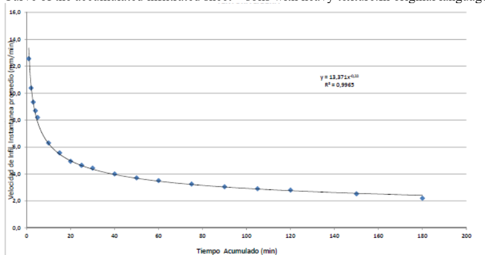
Figure 4. Average instantaneous infiltration rate curve – lightly textured soils. In original language Spanish
