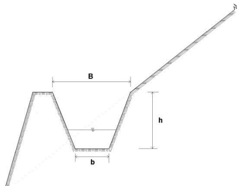
Section of an infiltration trench on a slope
