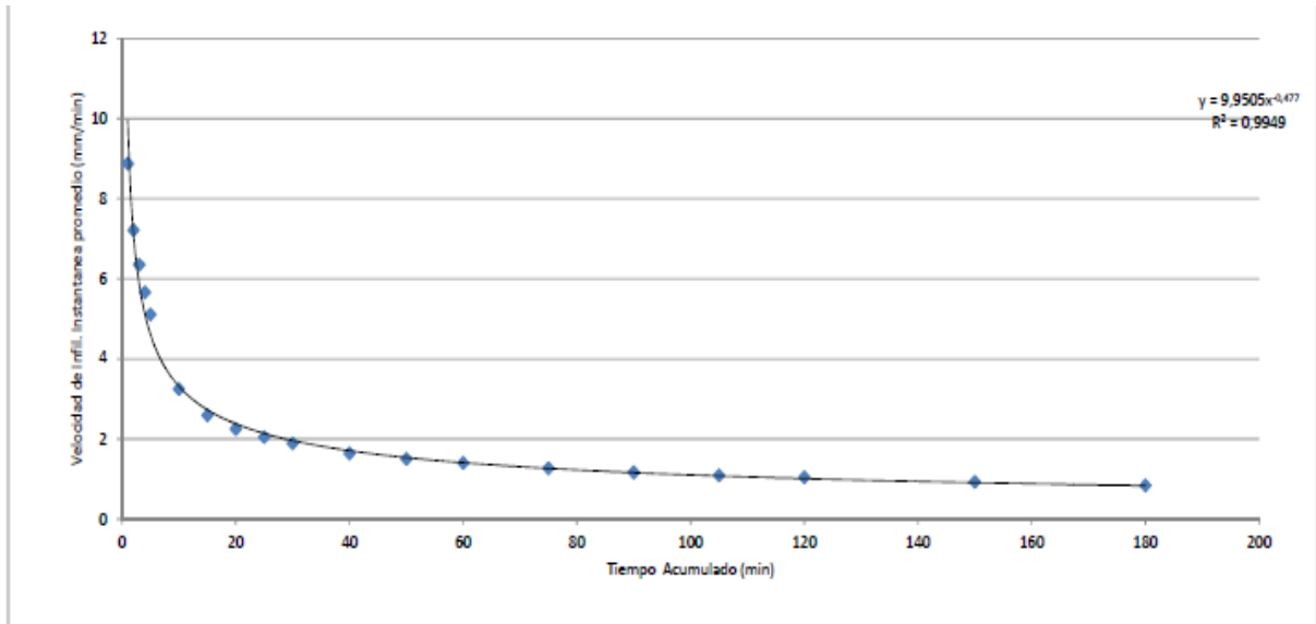
Figure 5. Average instantaneous infiltration rate curve – loamy textured soils. In original language Spanish
