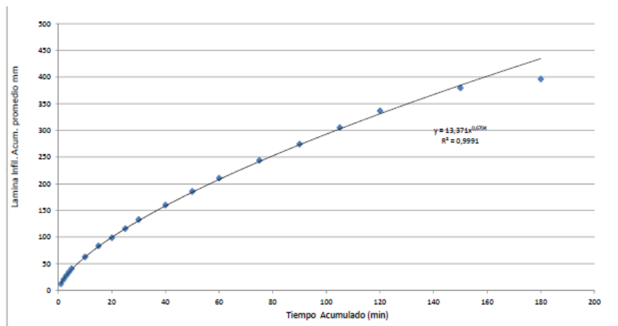
Figure 1. Curve of the average accumulated infiltrated sheet – lightly textured soils. In original language Spanish
