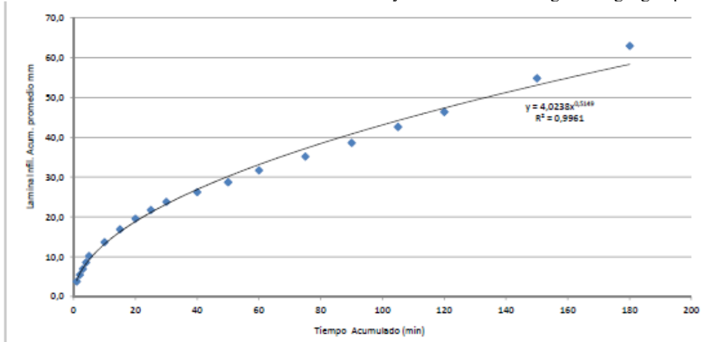
Figure 3. Curve of the accumulated infiltrated sheet – soils with heavy texture. In original language Spanish
