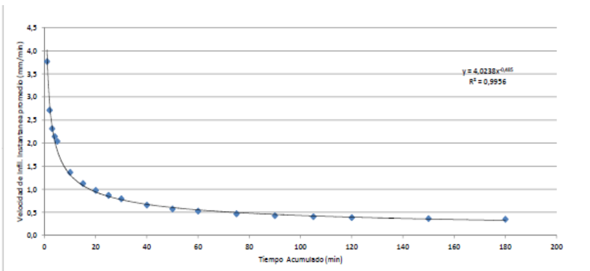
Figure 6. Average instantaneous infiltration rate curve – textured soils. In original language Spanish
