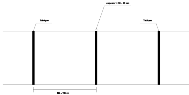
Plan views of an infiltration trench with partitions.
