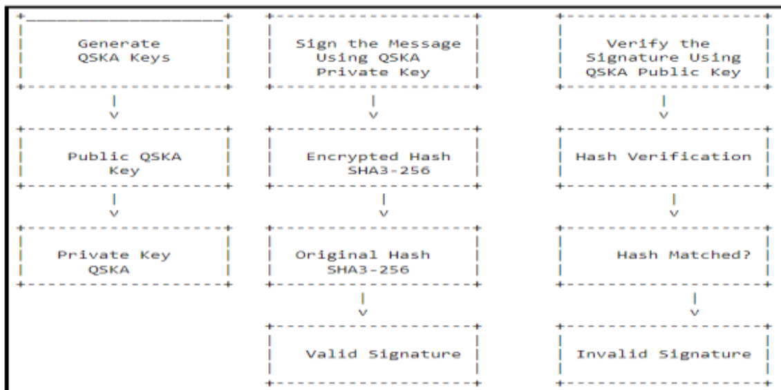
Figure (4) Architecture of Digital Signature in Python
