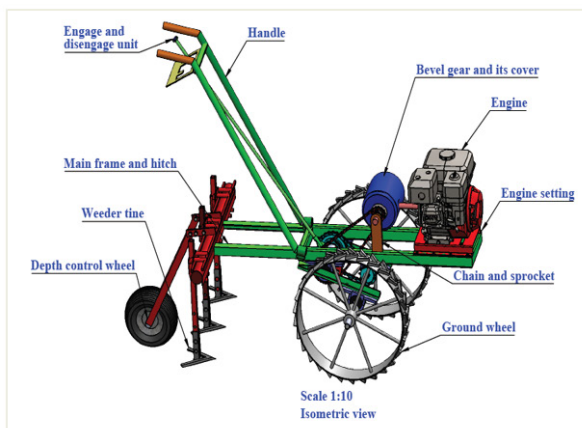
Figure 1: Weeding Machine
