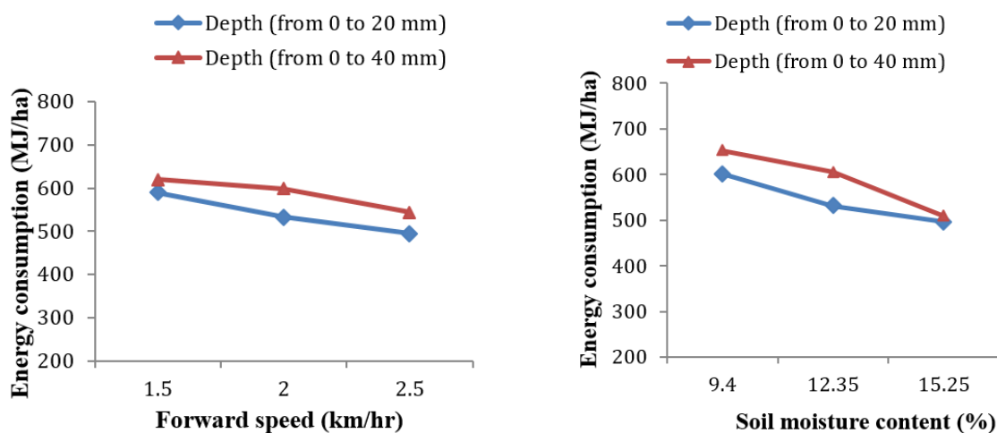
Figure 10: Effect of soil moisture and machine operational parameters on energy consumption
