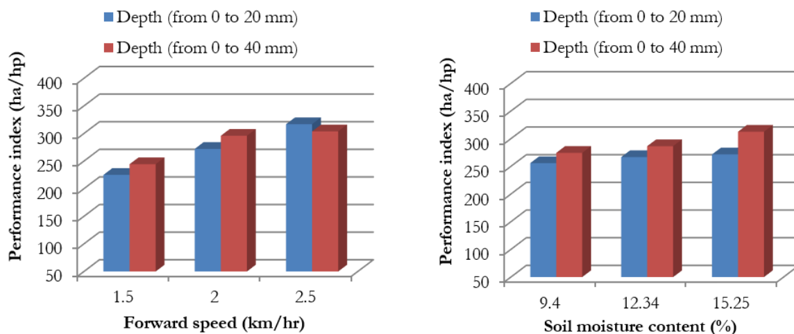
Figure 9: Effect of soil moisture and machine operational parameters on a performance index
