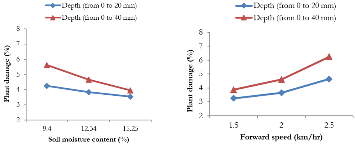
Figure 5: Effect of soil moisture and machine operational parameters on plant damage
