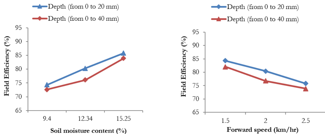
Figure 7: Effect of soil moisture and machine operational parameters on the field efficiency
