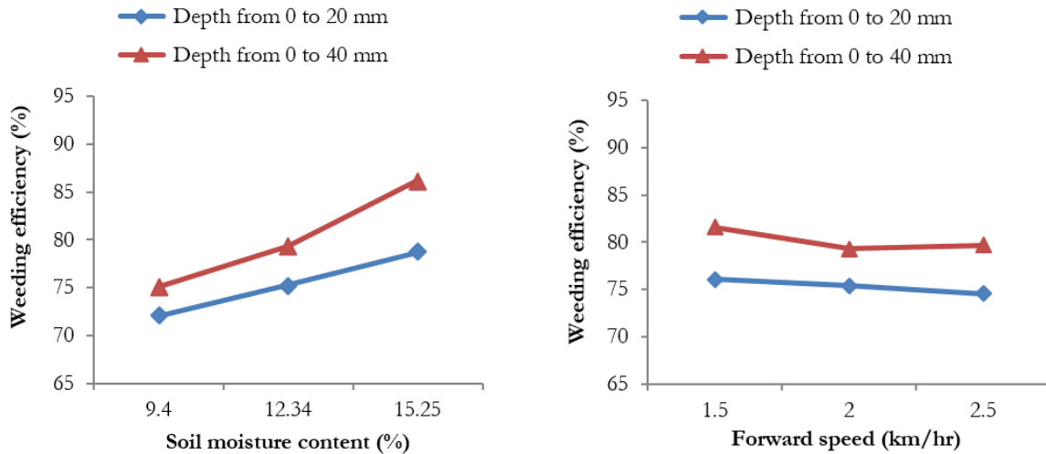
Figure 4: Effect of soil moisture and machine operational parameter weeding efficiency
