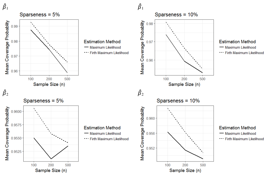
Figure 13. Estimated values of mean coverage probability ( CP ) for 95% confidence intervals for \beta_1 and \beta_2 for maximum likelihood and Firth maximum likelihood logistic regression models fitted using one binary predictor ( \beta_1 ) and one continuous predictor ( \beta_2 ) with either 5% sparseness or 10% sparseness
