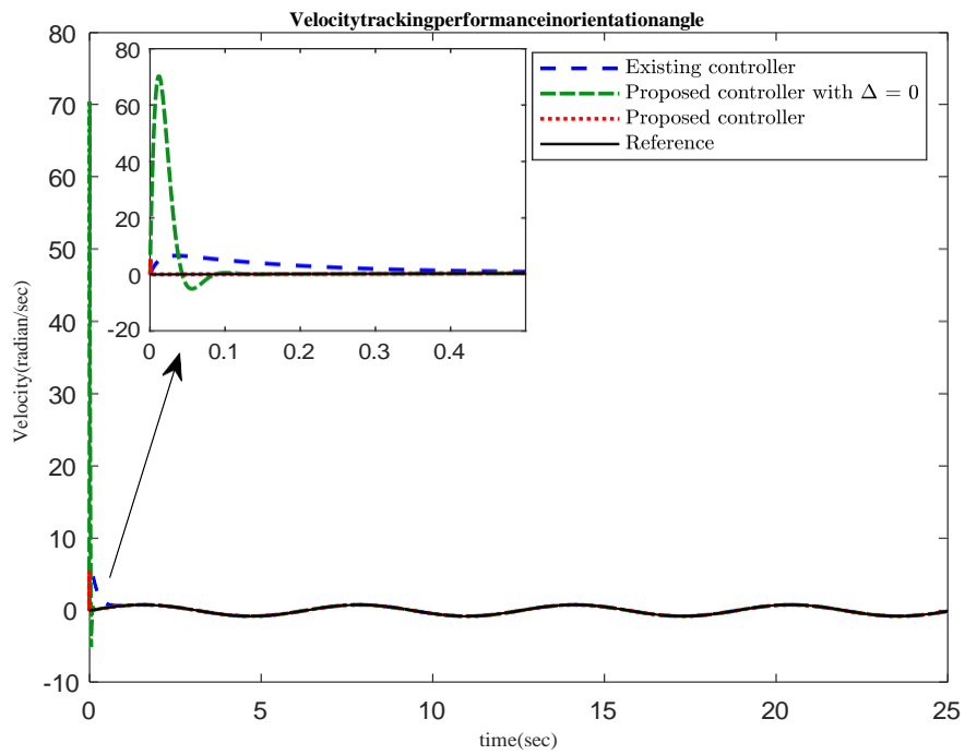
Fig.6.Velocity tracking performance for orientation angle
