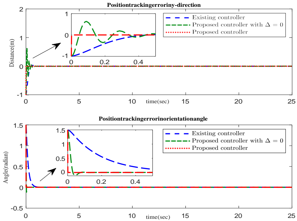
Fig.1.Position tracking errors
