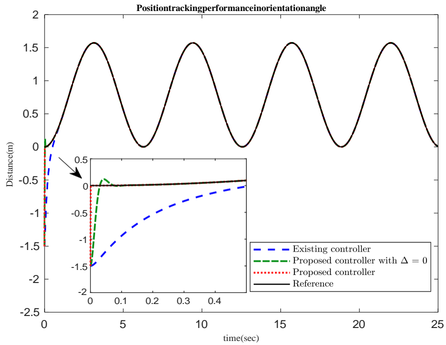
Fig.4.Position tracking performance for orientation angle
