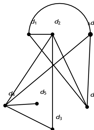
Figure 3.5. G_{\{d_1, d_2, d_5\}}
