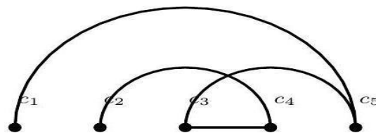
Figure 3.2. G_{\{c_1, c_3, c_4\}}
