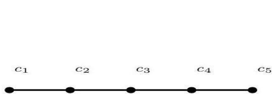
Figure 3.1. G = P_5
