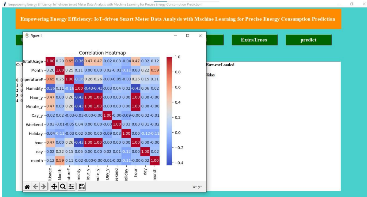
Figure 3: Correlation Heatmap
