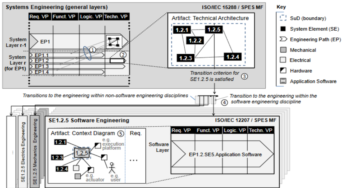
Figure 2- Integration ISO/IEC 15288- and ISO/IEC 12207-compliant engineering processes by using the SPES MF[5]
