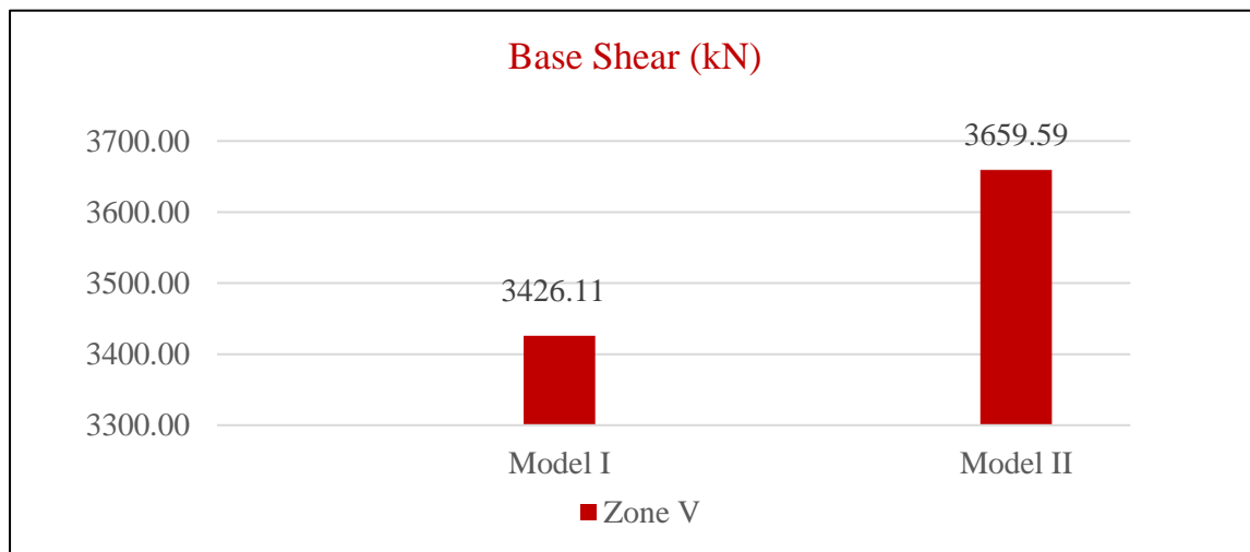
Figure 3: Base Shear X Direction & Z Direction
