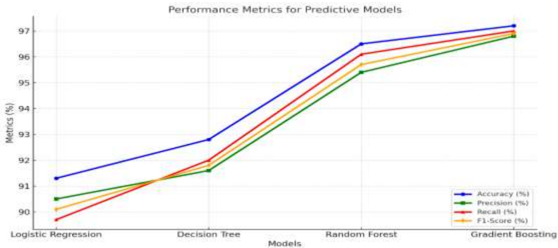
Figure 1: Performance Metrics for Predictive Models: A Comparative Analysis of Classification and Ensemble Models. The results presented in Figure 1 provide a detailed comparison of various machine learning models based on their performance metrics: accuracy, precision, recall, and F1-score. These metrics are critical for evaluating the reliability and effectiveness of models in predictive tasks, such as risk classification, dynamic pricing, and fraud detection within the insurance domain. The corresponding figure visually highlights the relative strengths of each model, aiding in understanding their comparative performance. Logistic Regression, a foundational classification model, achieves an accuracy of 91.3%, with precision, recall, and F1-score values of 90.5%, 89.7%, and 90.1%, respectively. These results indicate a balanced performance, making it a reliable choice for binary and multi-class classification tasks. However, its linear decision boundaries limit its effectiveness in capturing complex, non-linear relationships, leaving room for
