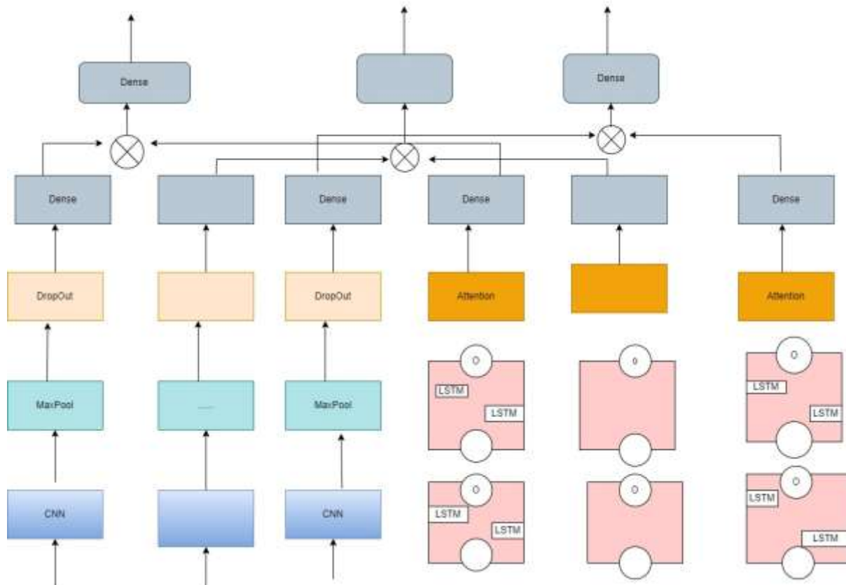
Architecture of BiLSTM
