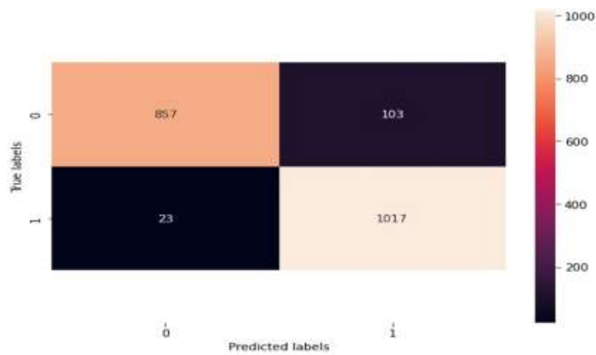
Figure.6. Confusion Metrics
