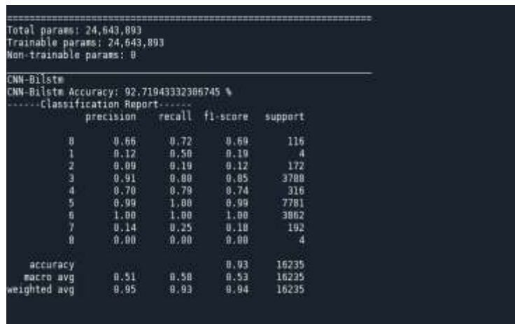
Figure.7. Modified Deep CNN-BiLSTM with AM Accuracy
