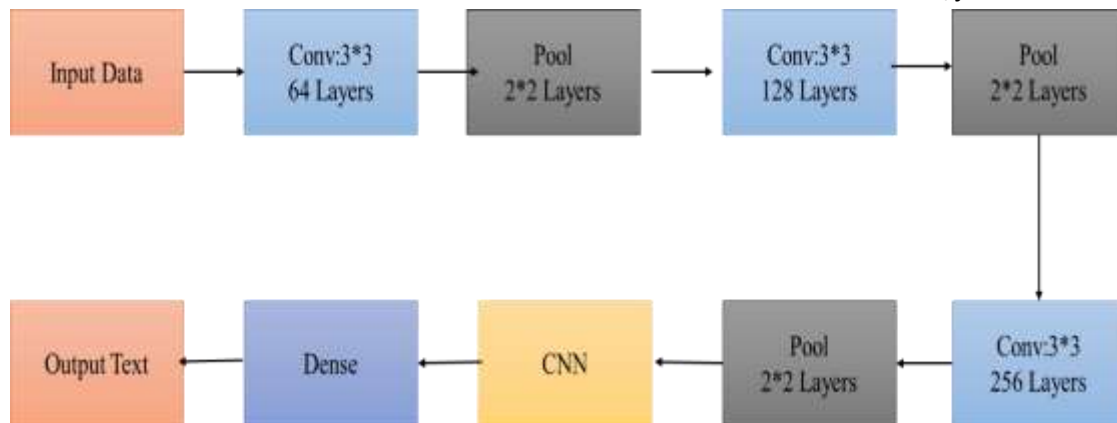
CNN Architecture
