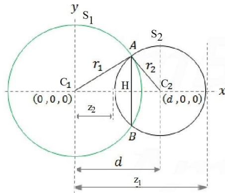
FIGURE2.IntersectingtwspheresS1andS2.
