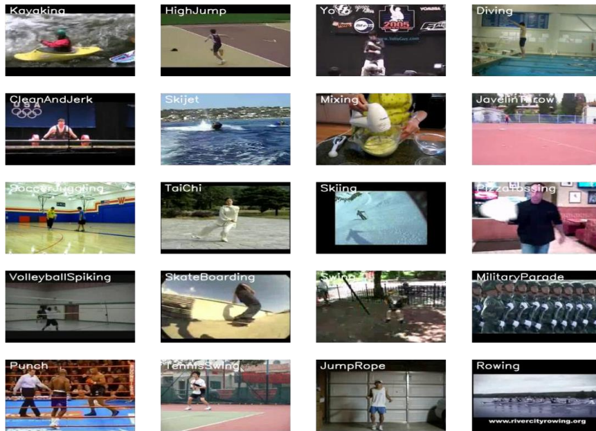
Fig3.UCF-50Dataset
