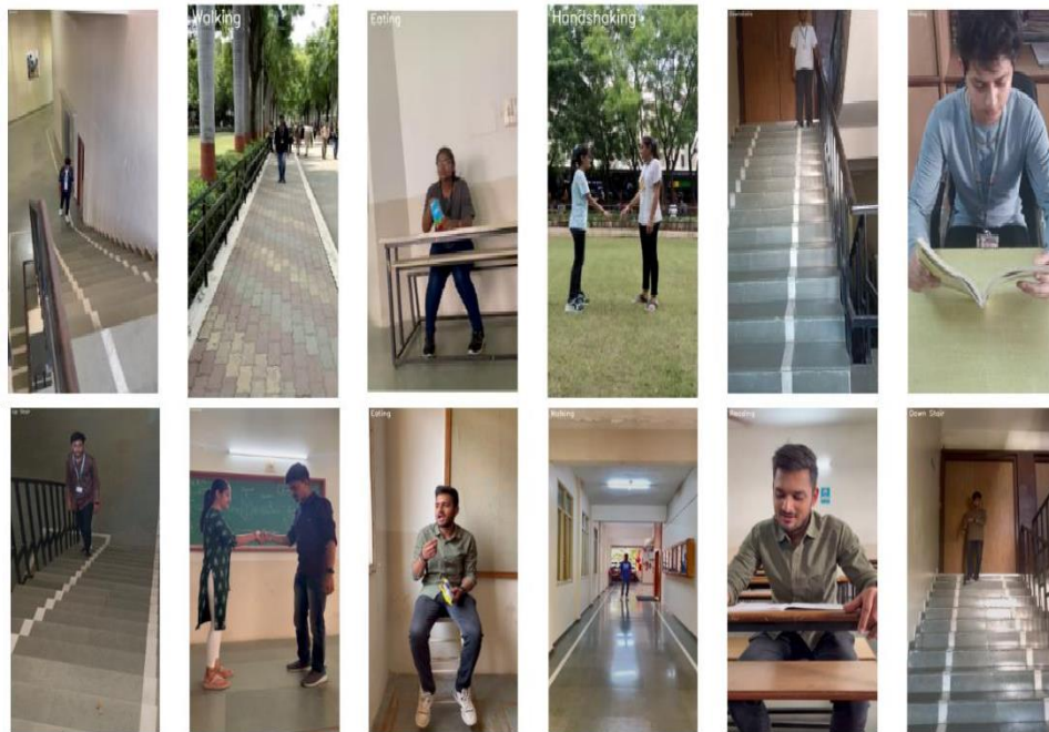
Fig4.OWN Dataset
