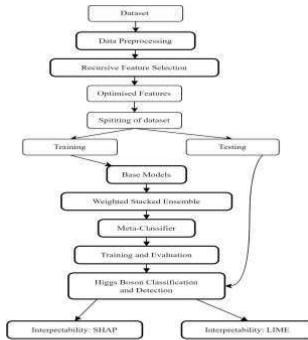
Fig. 1 Proposed Method for Explainable Higgs Bosson Detection and Classification
