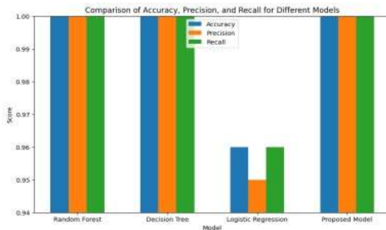
Figure 7: Comparison of the proposed method with the ML Techniques
