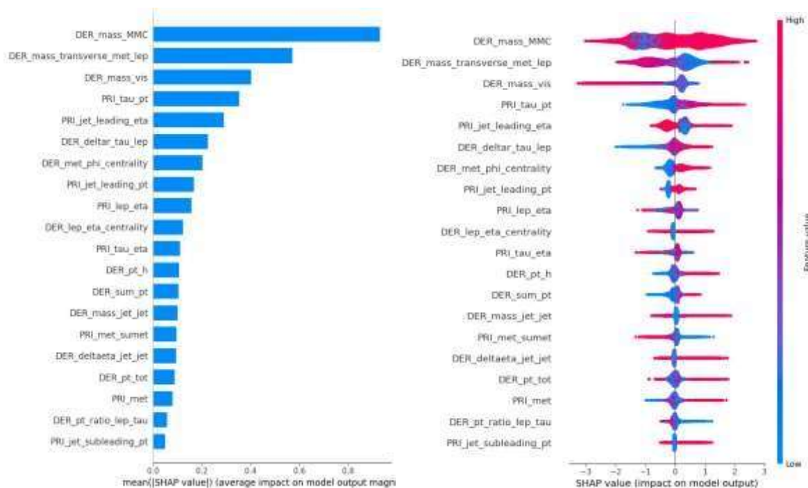
Figure 6: SHAP Feature Importance for Higgs Bosson Particles
