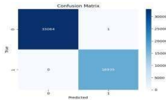
Figure 5: Confusion Metric for proposed Method
