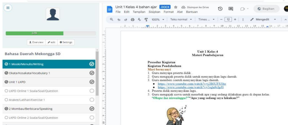
Figure4. Learning materials
