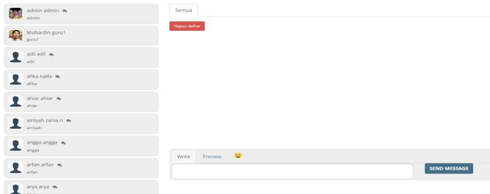
Figure5. Chat menu
