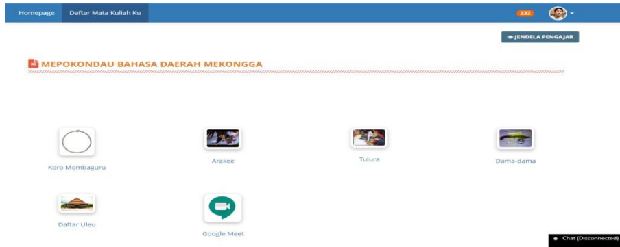
Figure3. Subject menu
