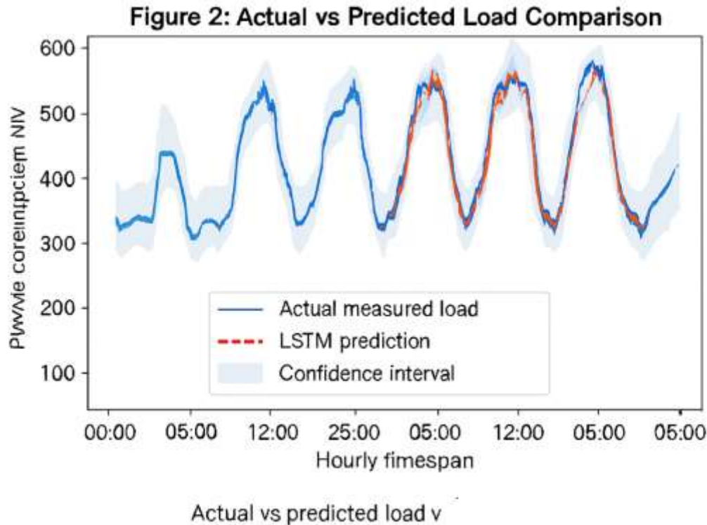
Figure 2: Actual vs Predicted Load Comparison
