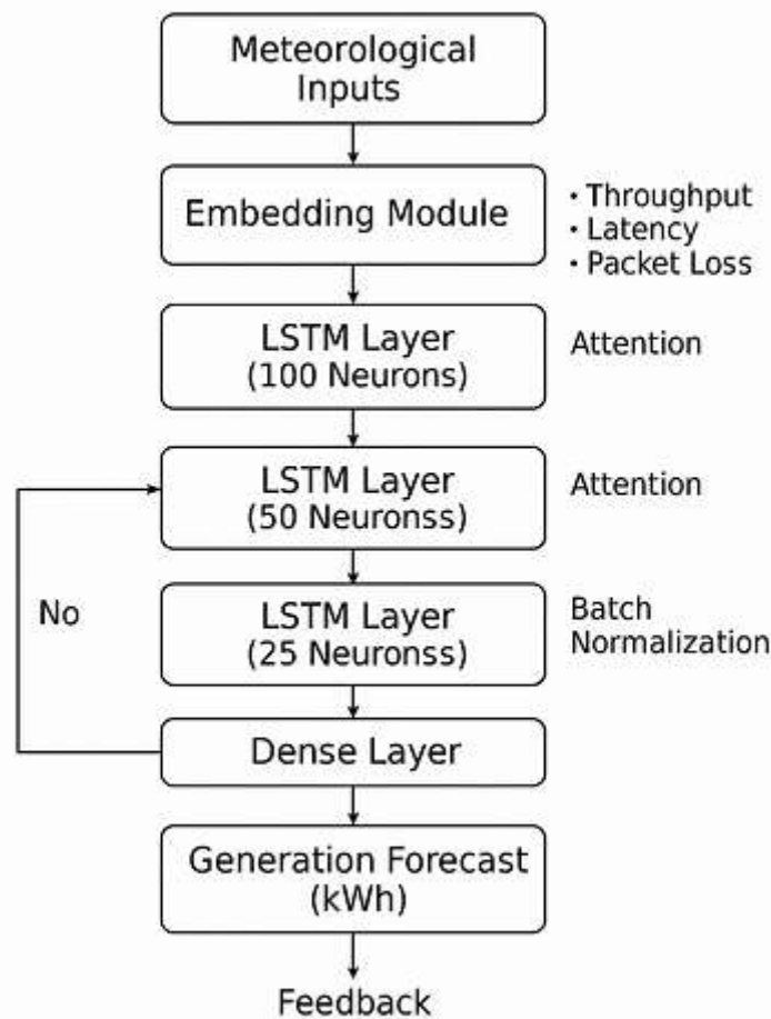
Figure 1: Solar Generation Forecasting Model Structure
