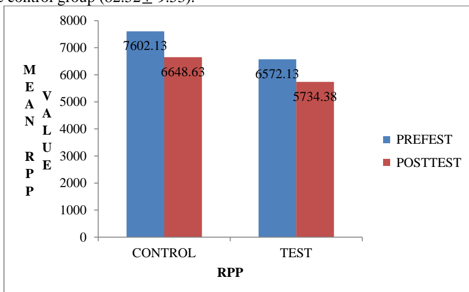
Fig.2. Bar chart showing RPP values for both control and test RPP= rate pressure product
