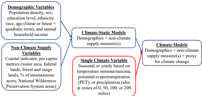
Figure 3. The process of modeling wherein the non-climate models are based on demographic and non-climate supply variable(s). After adding a single climate measure (proxy for climate change), the climate model projections can be compared against those from the non-climate models.
