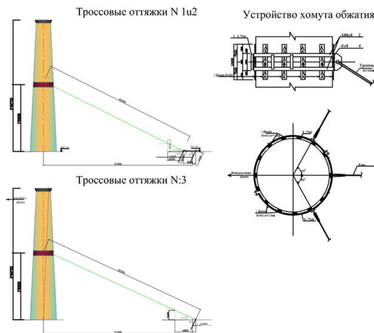
Figure 4. Elements of ‘iron belt’ project about construction of the minaret Saidniyoz Sholikorboy
