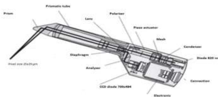
Figure 11. Scheme of Cerec 2 scanner head section
