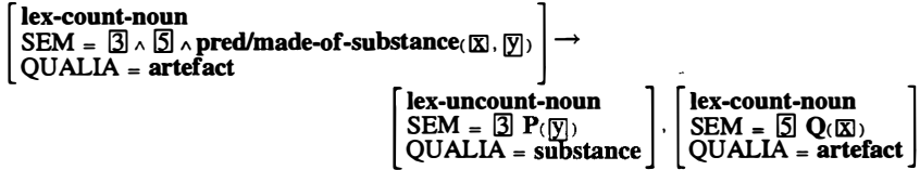
Figure 6: A compound noun subschema
