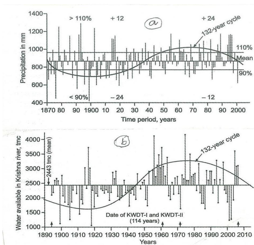
Figure 7: (a) Andhra Pradesh Annual Rainfall & (b) Annual Water Availability in Krishna River
