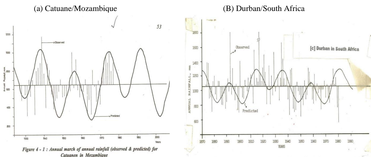
Figure 3 (a&b): Annual march of Rainfall [observed and predicted] (a) Catuane and (b) Durban
