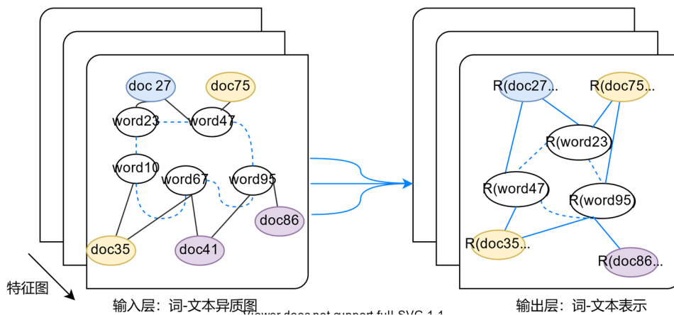
Figure 4. Flow diagram of the Text GCN model
