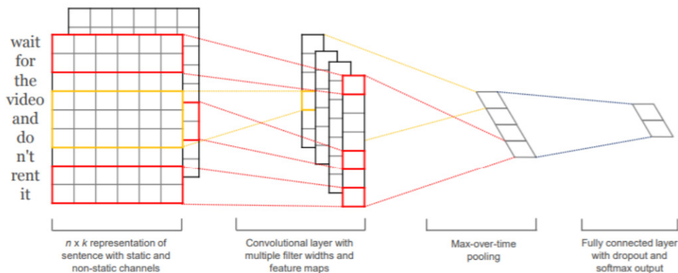
Figure 1. Structure of TextCNN network
