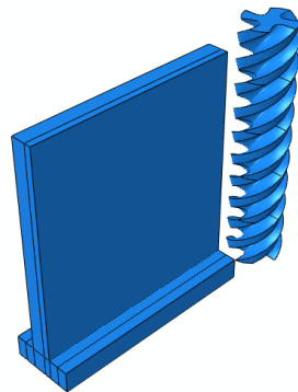
Fig 1. 3D orthogonal cutting model
