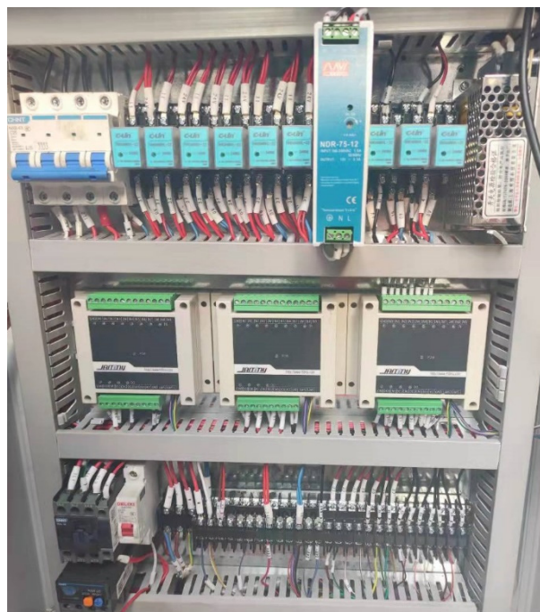
Figure 3. Control panel
