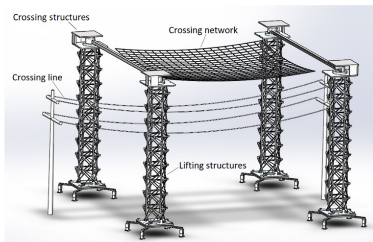
Figure 2. Crossing pole
