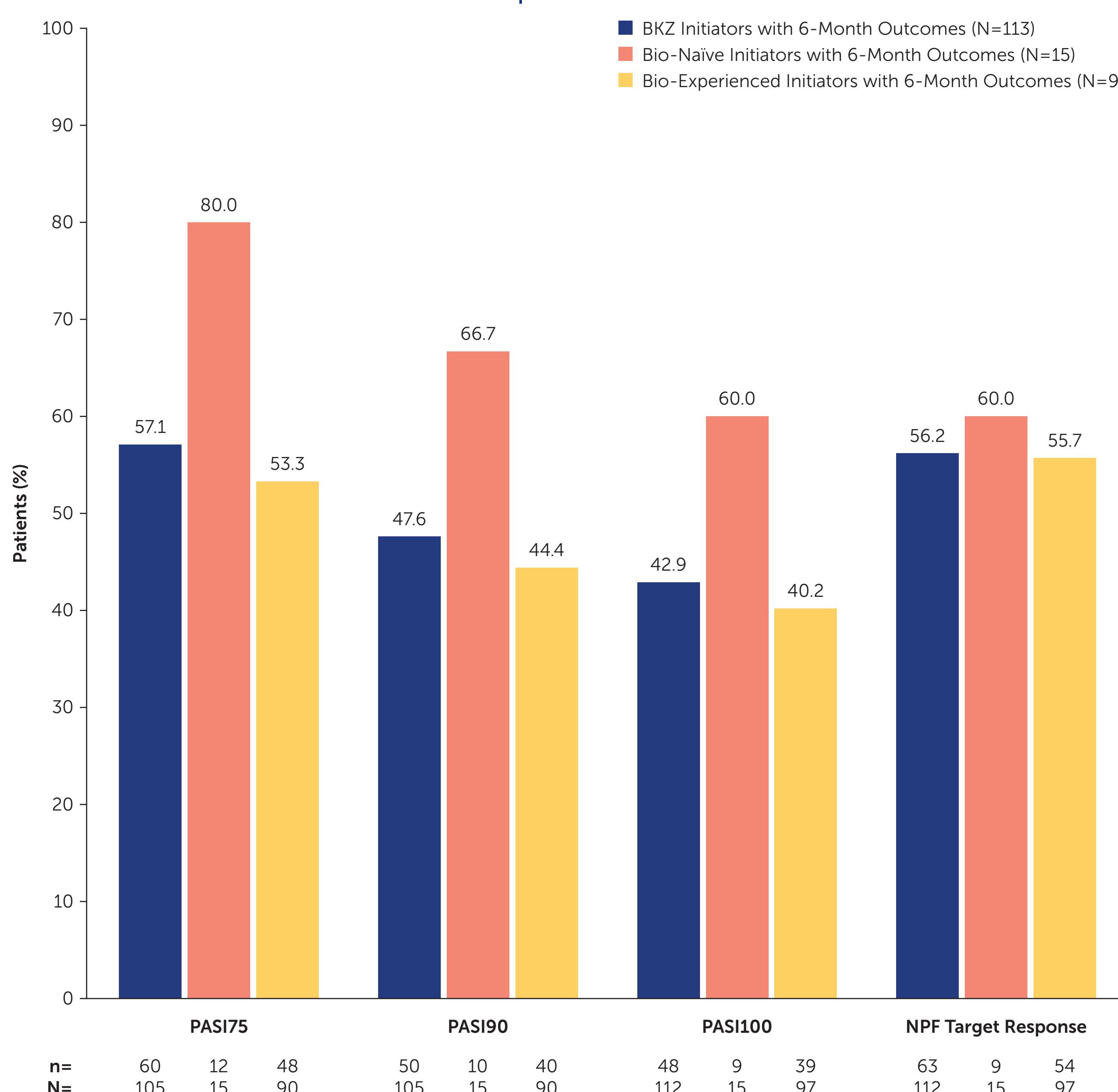
Figure 2 Proportion of patients achieving PASI responses at 6-month follow-up
