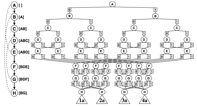
Figure 2: Context minimal graph (full caching)
