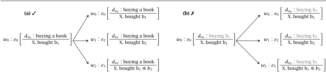
Figure 1 Actual decisions consistent (a) and inconsistent (b) with random choice modal component, assuming that the set of atomic books in the world of evaluation is \{b_1, b_2\} .
