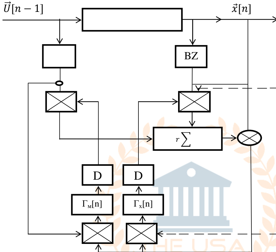
Fig.1. A discrete system that implements an adaptive identification algorithm for multiply connected objects in vector form.
