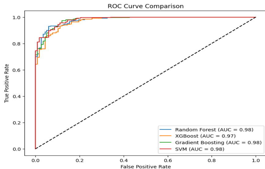
Figure 4. ROC Curve and AUC
