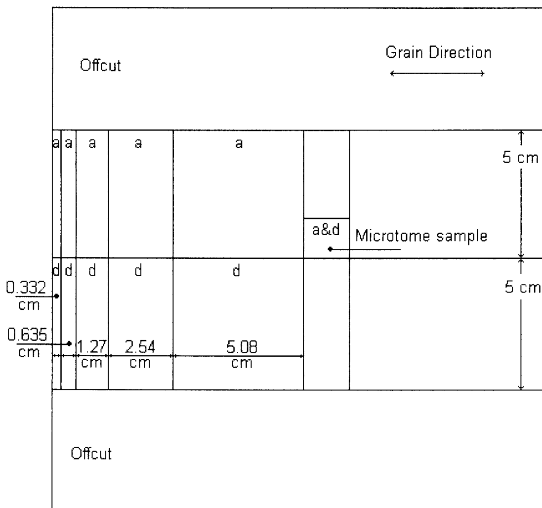
FIG. 1. Schematic illustrating the breakdown of each ~20-cm-long by ~20-cm-wide by 2.54-cm-thick section of red oak. a = adsorption, d = desorption.
