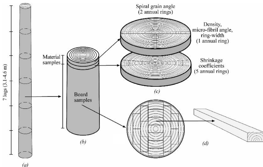
FIG. 2. Illustration of the experimental procedure, (a) Cutting pattern for experimental stems (20 trees); (b) Collection sample discs for material properties; (c) Cutting of discs for the material samples; (d) Saw pattern to produce individual boards.
